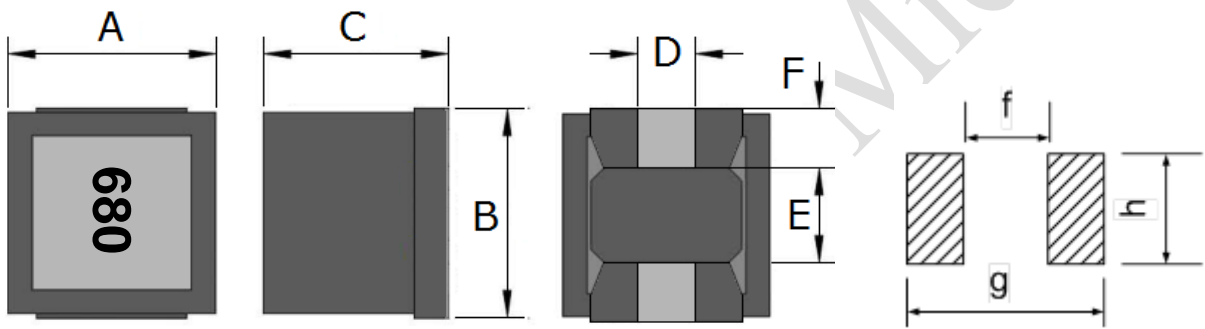
Recommended Land Pattern
